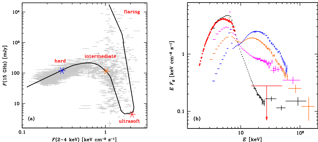
Fig. 1. Panel (a): Radio-X-ray track made by Cyg X-3 as it swings between different spectral states (data from Zdziarski et al. 2016 ). Panel (b): a set of average broadband spectra corresponding to the hard/radio quiescent (blue), intermediate/minor flaring (orange), ultrasoft/radio quenched (black), and soft non-thermal/flaring (magenta) states as introduced in Szostek et al. (2008) . IXPE data are shown with red symbols and the 2\sigma upper limit at 30 keV (in red) is from Swift/BAT.
