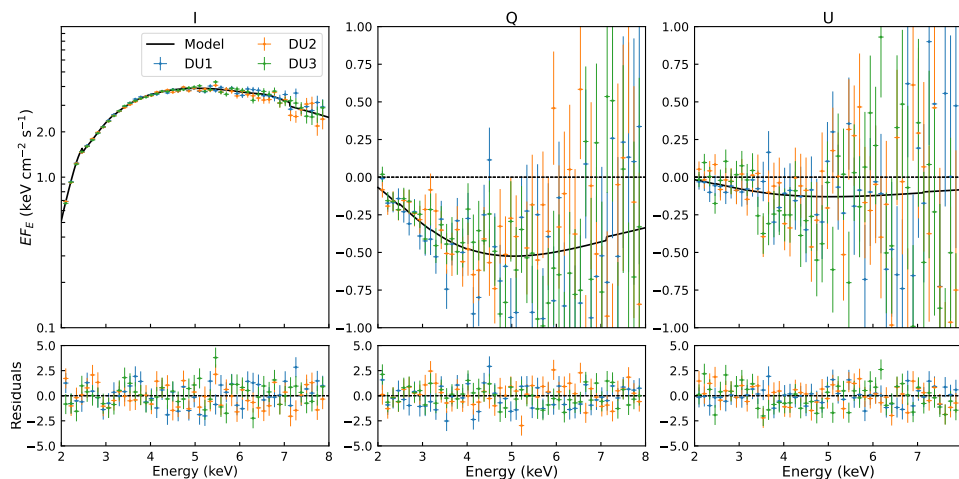
Fig. A.3. Same as Fig. A.1 but averaged over the orbital phases, during the time bins 2 and 3 (see Fig. 3).
