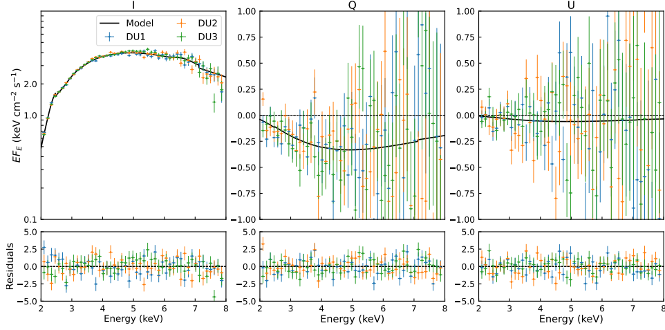
Fig. A.4. Same as Fig. A.1 but averaged over the orbital phases, during the time bin 5 (see Fig. 3).
